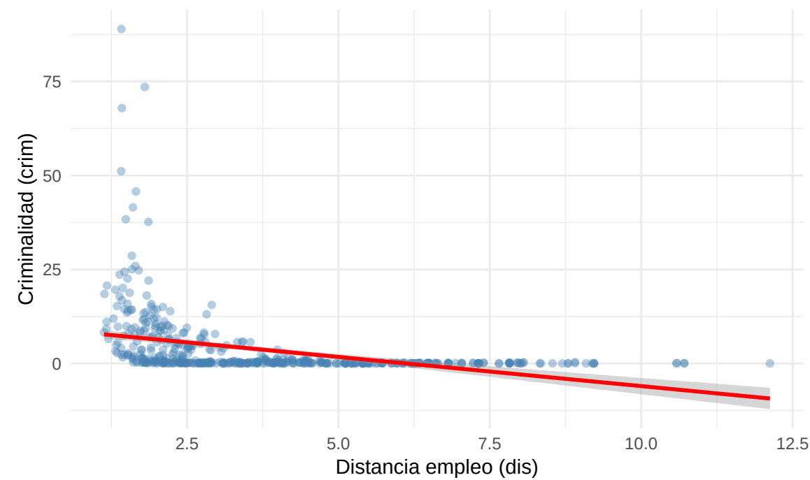
crim vs dis
